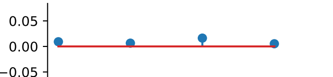
cross_orientation_correlation_magnitude
