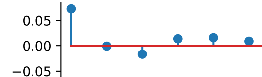
auto_correlation_reconstructed
