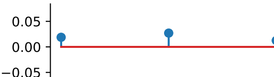
cross_scale_correlation_real
