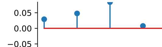
cross_scale_correlation_magnitude
