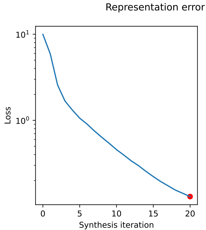
pixels+var_highpass
