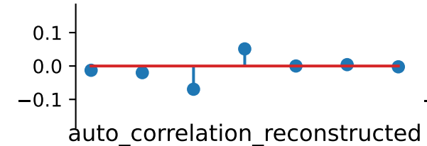
pixels+var_highpass
