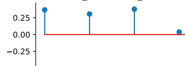
cross_scale_correlation_magnitude
