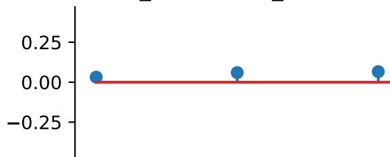
cross_orientation_correlation_magnitude
