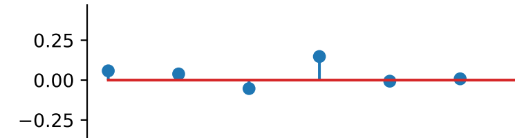
auto_correlation_reconstructed
