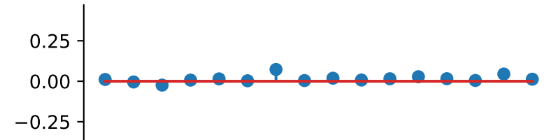
cross_orientation_correlation_magnitude
