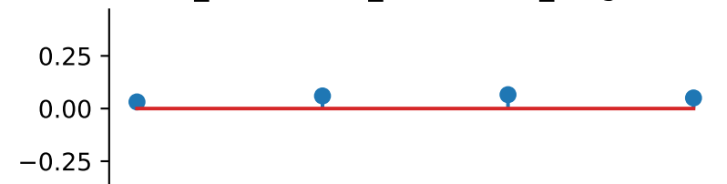
cross_orientation_correlation_magnitude
