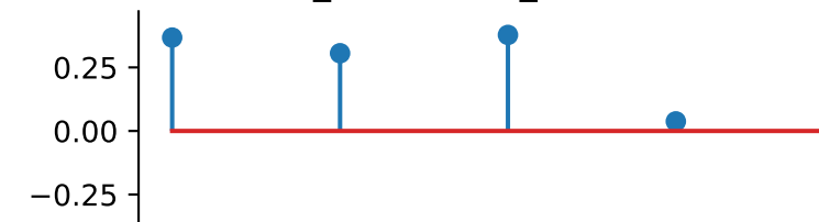
cross_scale_correlation_magnitude
