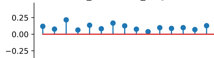
cross_scale_correlation_real
