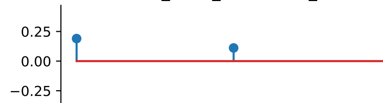
cross_scale_correlation_real
