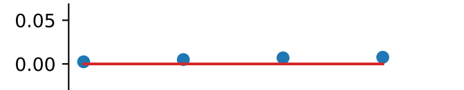
cross_orientation_correlation_magnitude
