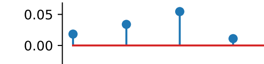
auto_correlation_reconstructed
