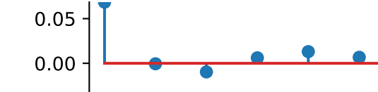
pixels+var_highpass
