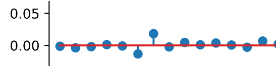
std+skew+kurtosis recon
