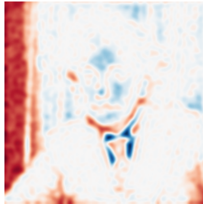
Representation error_00 range: [-2.1\text{e-}01, 2.1\text{e-}01] dims: [256, 256] * 1.0
