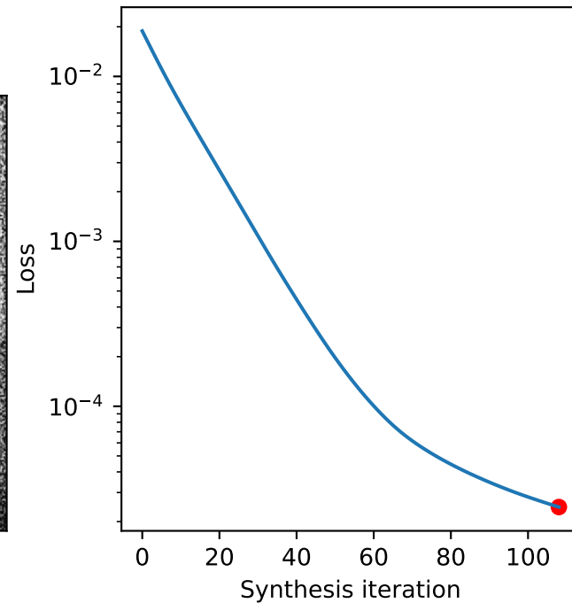
Metamer[0] [iteration=108] range: [-3.8\text{e-}04, 1.0\text{e+}00] dims: [256, 256] * 1.0
