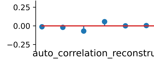
pixels+var_highpass
