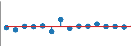
std+skew+kurtosis recon
