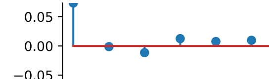
pixels+var_highpass
