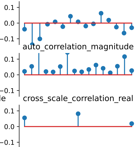
std+skew+kurtosis recon
