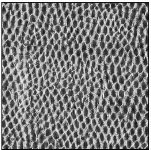
Metamer [iteration=20] range: [2.2e-03, 1.0e+00] dims: [256, 256] * 1.0
