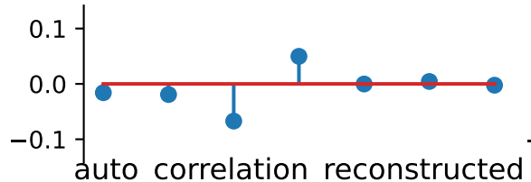
pixels+var_highpass
