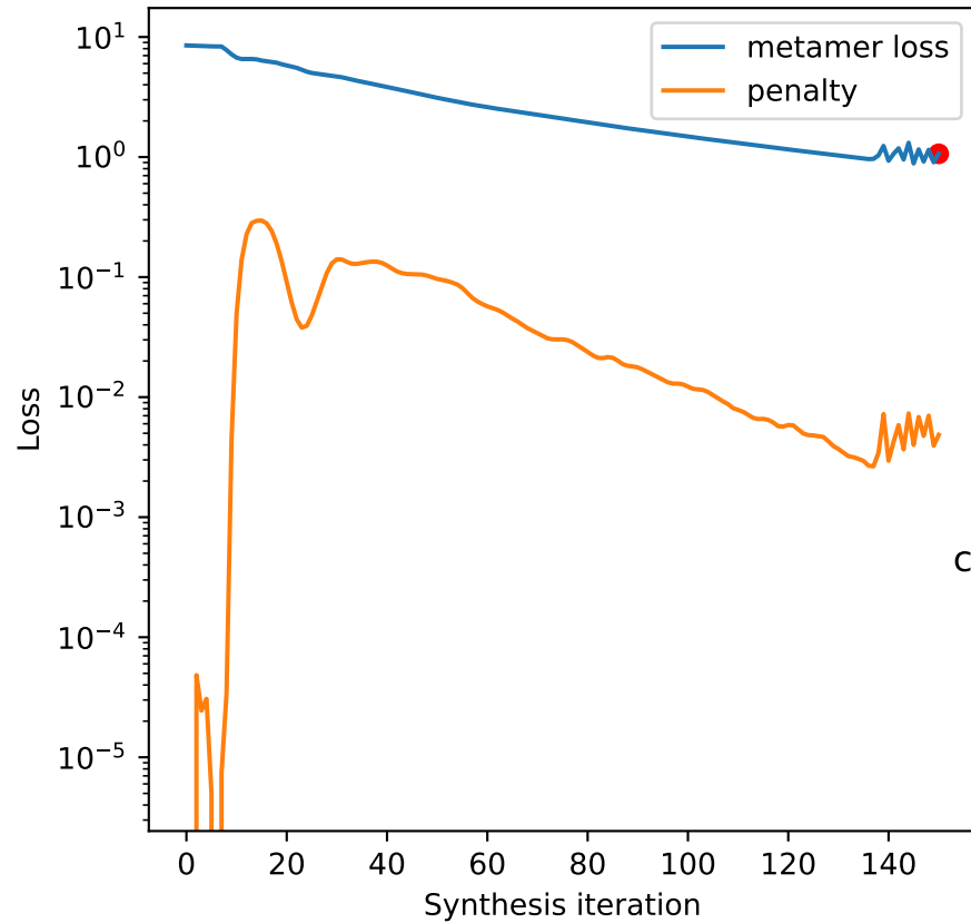
Representation error
