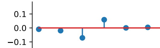
pixels+var_highpass
