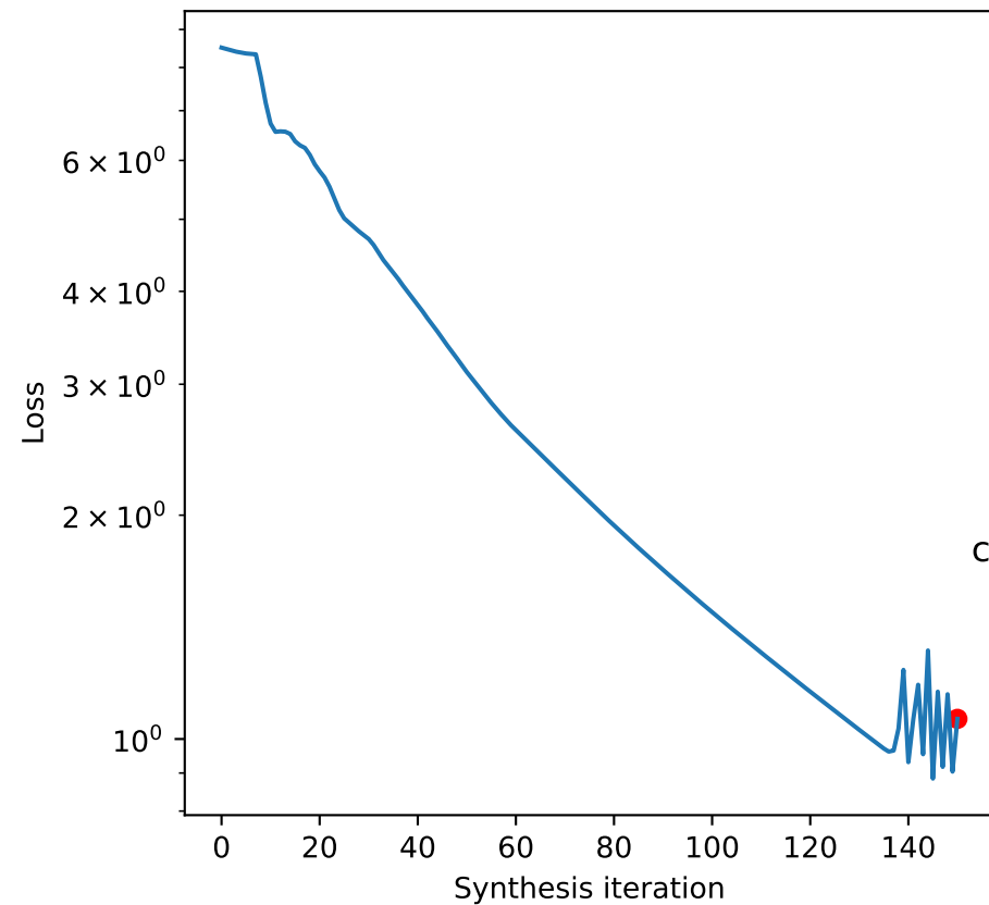
Representation error
