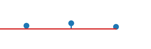
cross_orientation_correlation_magnitude
