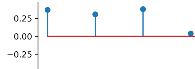
cross_scale_correlation_magnitude
