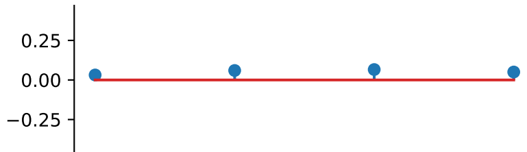
cross_orientation_correlation_magnitude
