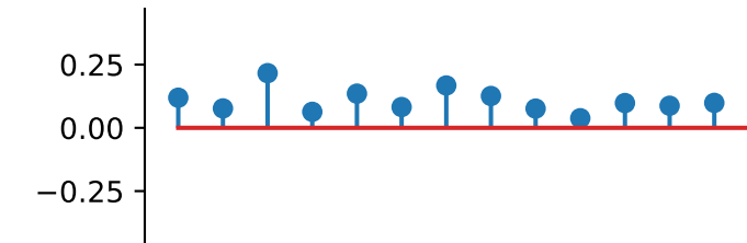
cross_scale_correlation_real
