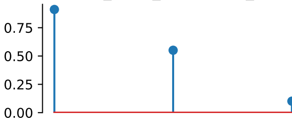
cross_scale_correlation_real
