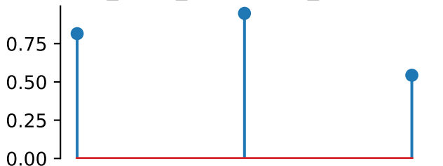
cross_scale_correlation_magnitude
