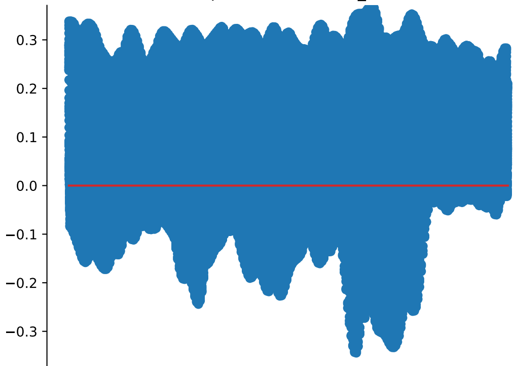
Representation error_00
