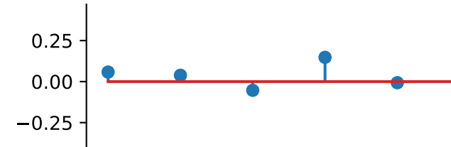
auto_correlation_reconstructed
