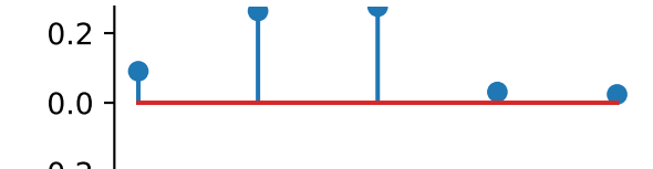
cross_scale_correlation_magnitude
