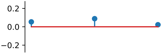
cross_scale_correlation_real
