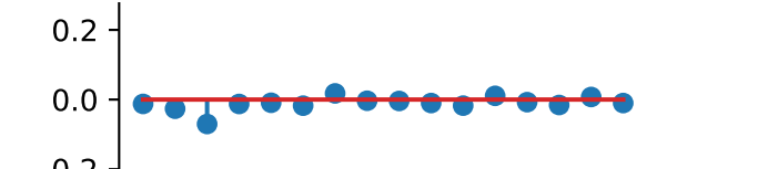
cross_orientation_correlation_magnitude
