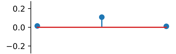
cross_scale_correlation_magnitude
