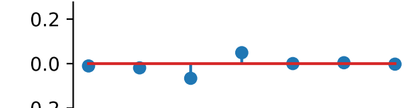
auto_correlation_reconstructed
