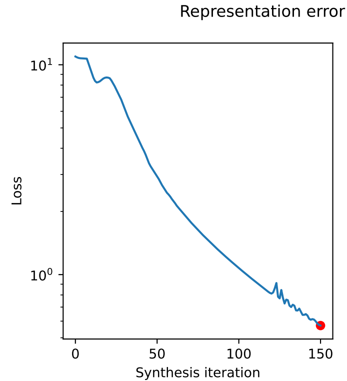
pixels+var_highpass
