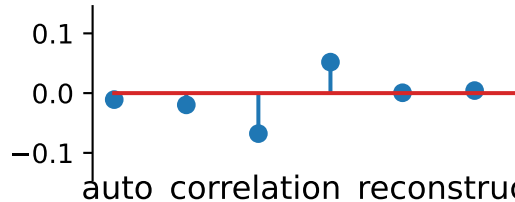
pixels+var_highpass
