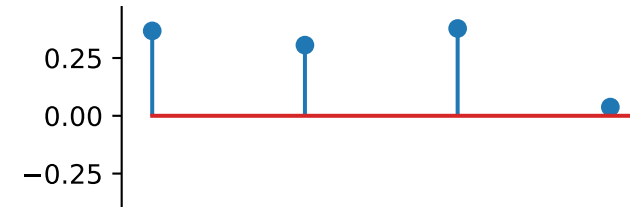
cross_scale_correlation_magnitude
