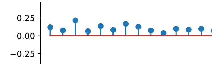
cross_scale_correlation_real
