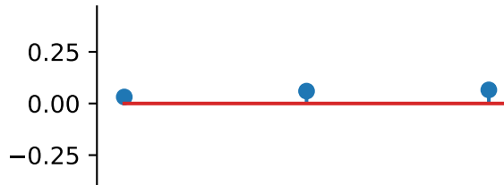
cross_orientation_correlation_magnitude
