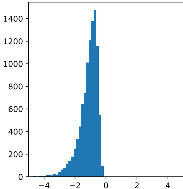
Left skew: -1.6936
