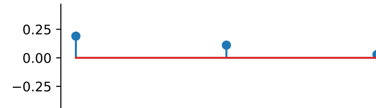
cross_scale_correlation_real
