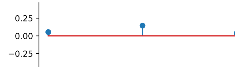
cross_scale_correlation_magnitude
