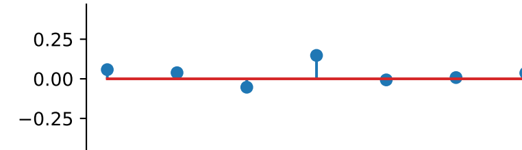
auto_correlation_reconstructed
