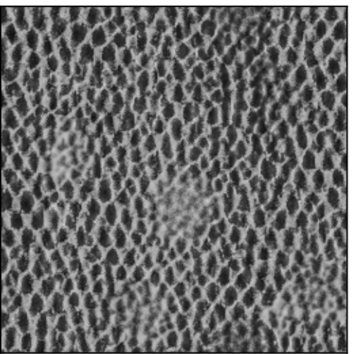
Metamer[0] [iteration=150] range: [-3.4e-04, 1.0e+00] dims: [256, 256] * 1.0
