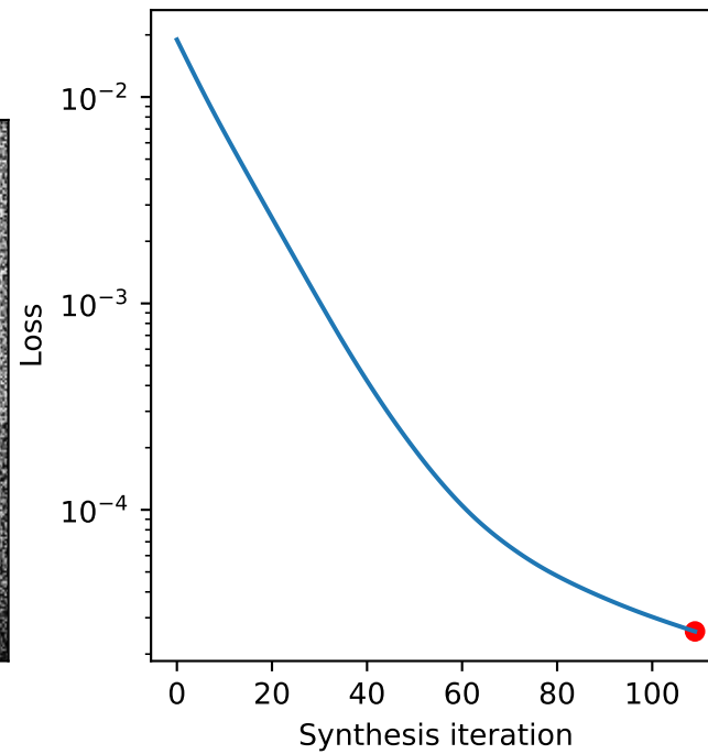
Metamer[0] [iteration=109] range: [-6.1\text{e-}04, 1.0\text{e+}00] dims: [256, 256] * 1.0
