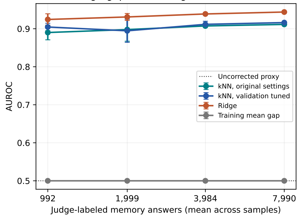
High-gap AUROC (higher is better)
