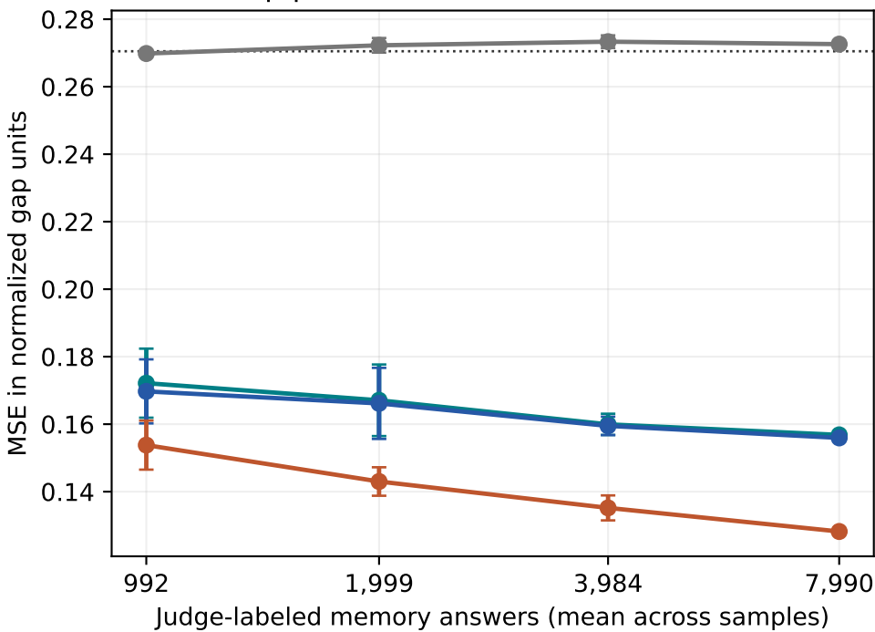
Gap prediction error (lower is better)
