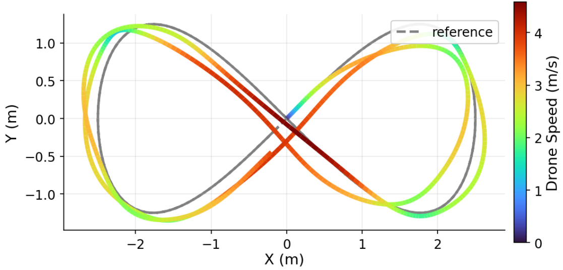
Figure 4: Flown path of the fastest champion at 4.0 \text{ m s}^{-1} , coloured by speed, against the reference
