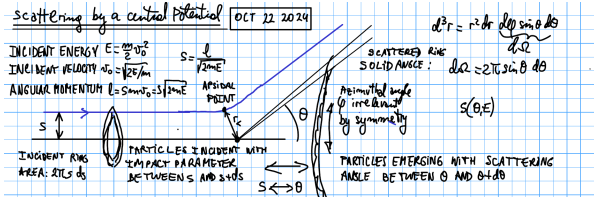
Figure 1: Impact-parameter and scattered-ring geometry: particles incident with impact parameter between s and s + ds (left) emerge with scattering angle between \theta and \theta + d\theta into the ring of solid angle d\Omega (right). The azimuthal angle \varphi is irrelevant by the symmetry of a central potential, so the scattering problem reduces to a function s = S(\theta, E) .
