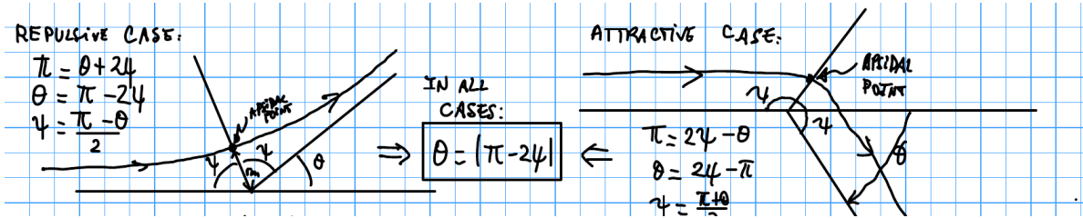
Figure 2: Repulsive case ( \pi = \theta + 2\psi , left) and attractive case ( \pi = 2\psi - \theta , right); \psi is the angle at the apsidal point between the incoming asymptote and the line to the force center.
