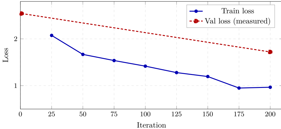
Figure 2: LoRA SFT training dynamics. Training loss (filled line) is logged each 25 iters; validation loss (dashed) is measured at iter 1 and iter 200. The 32% validation-loss reduction over 200 iters corresponds to a substantial qualitative shift in generations.
