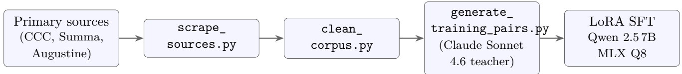
Figure 1: End-to-end data pipeline for Phase 1. Primary sources are scraped respectfully, cleaned into a structured JSONL chunk corpus, then expanded by a Claude Sonnet 4.6 teacher into (question, scholastic-answer) pairs that drive LoRA SFT of Qwen 2.5 7B-Instruct under MLX with 8-bit weight quantization.
