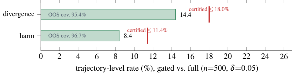
Figure 5: E10: the trajectory-level certificate. Green bars are the empirical rates (gated vs. full); red ticks are the certified (1 - \delta) upper bounds. Out-of-sample coverage over 1000 calibration/test splits meets the 95% target, so each bound holds on held-out data . “Harm” = a task full context solved that the compressed run did not.
