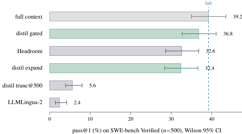
Figure 4: E8 frontier: task-success of every condition (pass@1 with Wilson 95% intervals, n=500 , identical 30-turn ReAct agent, official harness). Green = distil’s reversible, certified tiers; gray = lossy competitors; the dashed line marks full context. distil’s relevance-gated tier is the highest-accuracy compressor and the only one whose interval overlaps full; both lossy token-droppers collapse.
