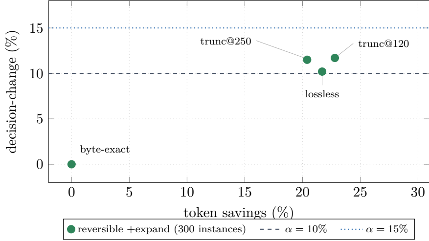
Figure 3: E1 frontier on full real SWE-bench_Lite (300 instances, 600 decisions; Claude grader, majority-of-3 structured, +expand recovery loop). The reversible digest at 21.7% savings achieves 10.2% decision-change, beating equally-aggressive lossy truncation (11.5–11.7%) at \approx 22\% savings. On a 40-instance subset the recovery effect is sharper (11.2% no-expand \rightarrow 7.5% with +expand; see Figure 4). Dashed lines show the \alpha = 10\% and \alpha = 15\% risk budgets. \tau -bench airline (25 traj, 105 decisions) is not plotted: the data is already compact (lossless saves only 1.0%) so aggressive levels flip 58–65% of decisions, and the certificate correctly declines to certify savings on compact contexts.
