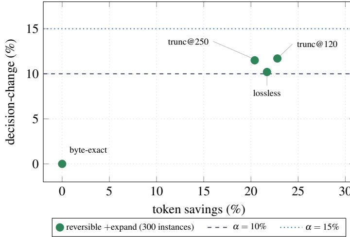
Figure 3: E1 frontier on full real SWE-bench_Lite (300 instances, 600 decisions; Claude grader, majority-of-3 structured, +expand recovery loop). The reversible digest at 21.7% savings achieves 10.2% decision-change, beating equally-aggressive lossy truncation (11.5–11.7%) at \approx 22\% savings. On a 40-instance subset the recovery effect is sharper (11.2% no-expand \rightarrow 7.5% with +expand; see Figure 4). Dashed lines show the \alpha = 10\% and \alpha = 15\% risk budgets. \tau -bench airline (25 traj, 105 decisions) is not plotted: the data is already compact (lossless saves only 1.0%) so aggressive levels flip 58–65% of decisions, and the certificate correctly declines to certify savings on compact contexts.
