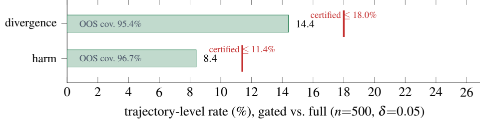
Figure 8: E10: the trajectory-level certificate. Green bars are the empirical rates (gated vs. full); red ticks are the certified (1 - \delta) upper bounds. Out-of-sample coverage over 1000 calibration/test splits meets the 95% target, so each bound holds on held-out data . “Harm” = a task full context solved that the compressed run did not.
