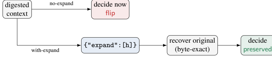
Figure 4: Expand-aware grading. Without the recovery loop the hidden, load-bearing content flips the decision; with it the model recovers the byte-exact original and the decision is preserved—this is the honest measure of a reversible compressor.
