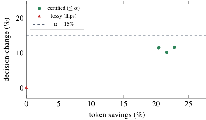
Figure 6: E1 certified frontier on the SWE-bench headline run (real grader).
