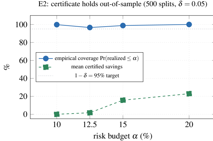
Figure 5: E2: out-of-sample certificate validity on full real SWE-bench_Lite (+expand, 300 instances, 500 splits, \delta = 0.05 ). Blue solid: empirical coverage \Pr(\text{realized risk} \leq \alpha) —96.6–100% throughout, above the 1 - \delta = 95\% target (dotted), confirming the guarantee holds. Green dashed: mean certified savings, which rises sharply from 1.7% at \alpha = 12.5\% to 15.7% at \alpha = 15\% and 22.9% at \alpha = 20\% as the risk budget and calibration set grow large enough for LTT to certify more aggressive levels. The certificate is conservative: realized risk at \alpha = 15\% is 8.0%, well below the budget.
