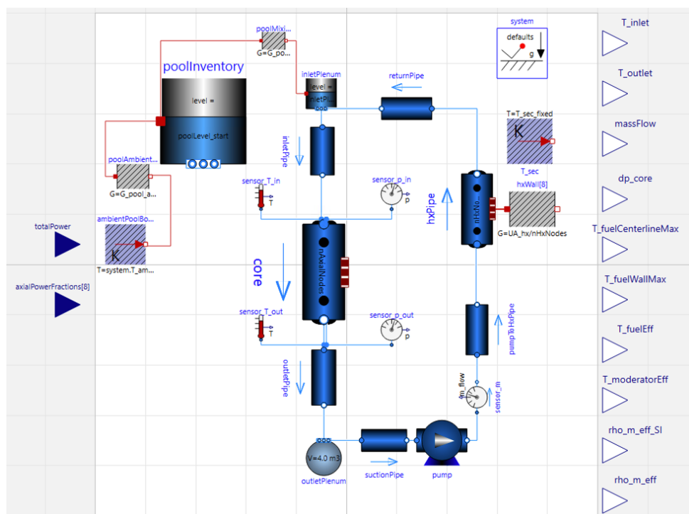
Figure 1: Modelica primary-loop and core thermal-hydraulics model.
