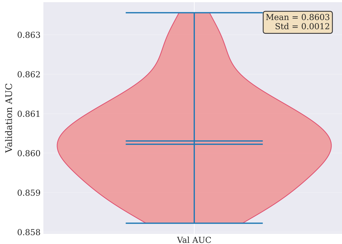
(b) Violin Plot
