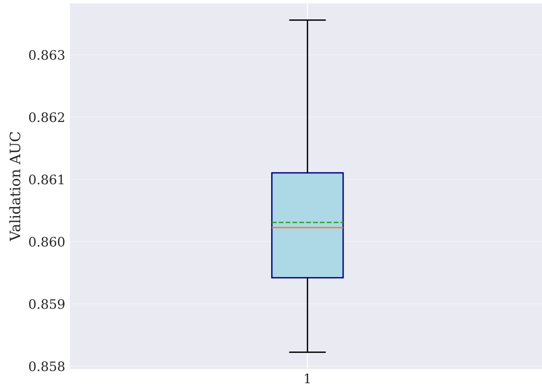
(a) Box Plot
