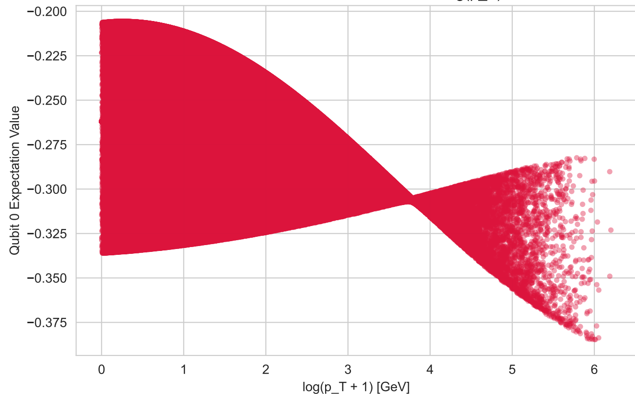
Kinematic Correlation: Qubit 0 vs \log(p_T)
