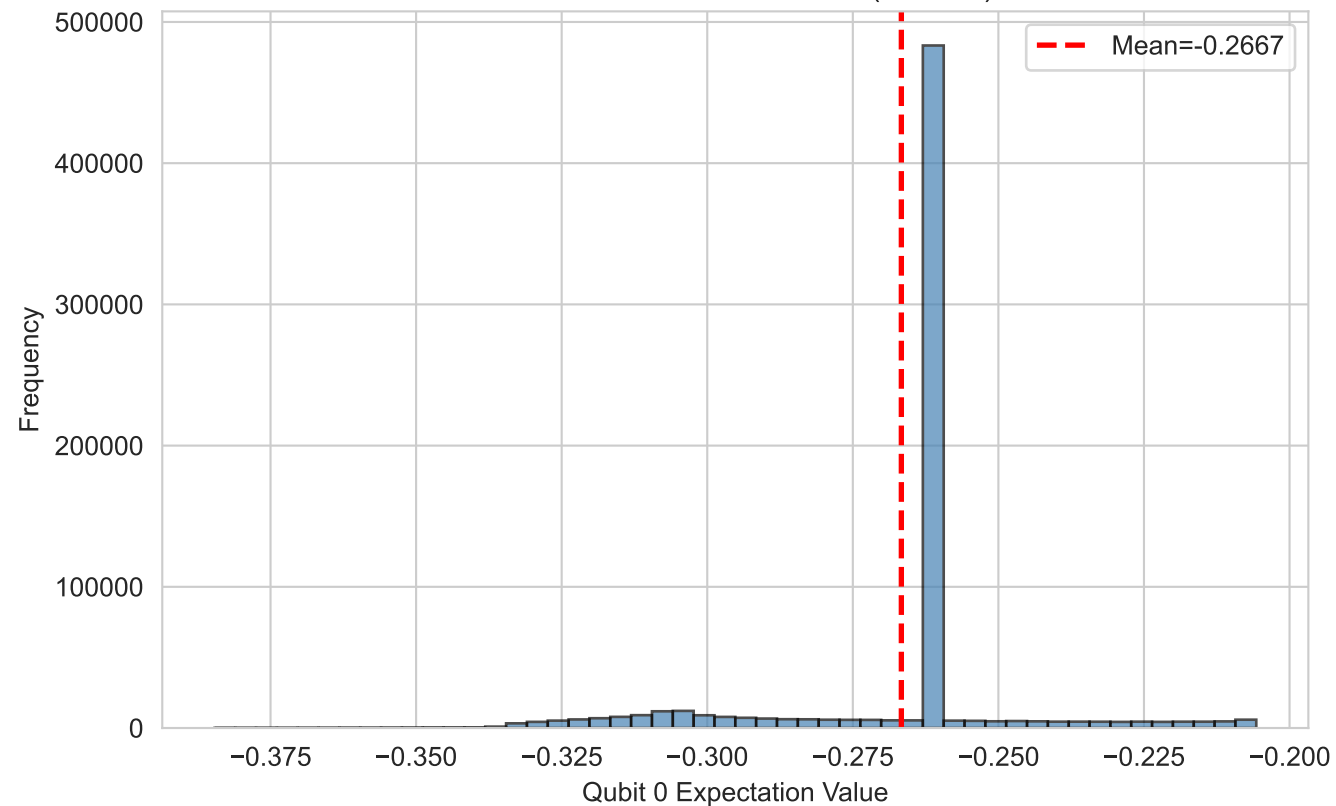
Quantum State Distribution (Qubit 0)
