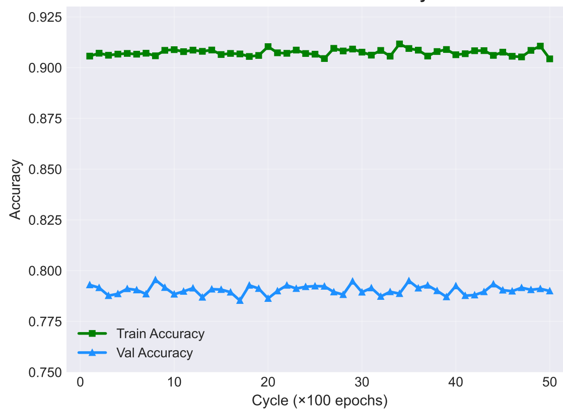
Train vs Validation Accuracy
