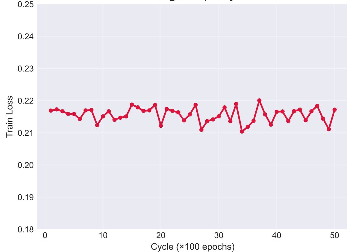
Training Loss per Cycle
