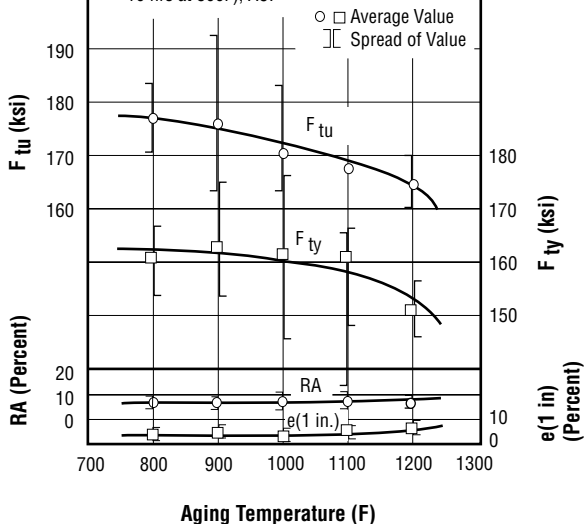
Figure 3.2.1.11 Effect of aging temperatures on tensile properties of three compressor casings cast from one heat (Ref. 4)
