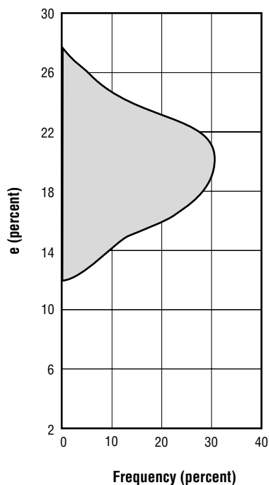
Figure 3.2.1.6 Frequency distribution of tensile properties of hot isostatically pressed and annealed T1-6Al-4V casting test bars from 500 heats (Ref. 24)
