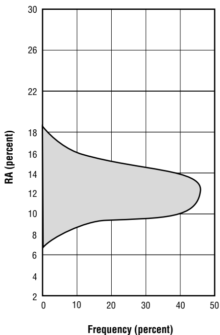
Figure 3.2.1.6 Frequency distribution of tensile properties of hot isostatically pressed and annealed T1-6Al-4V casting test bars from 500 heats (Ref. 24)
