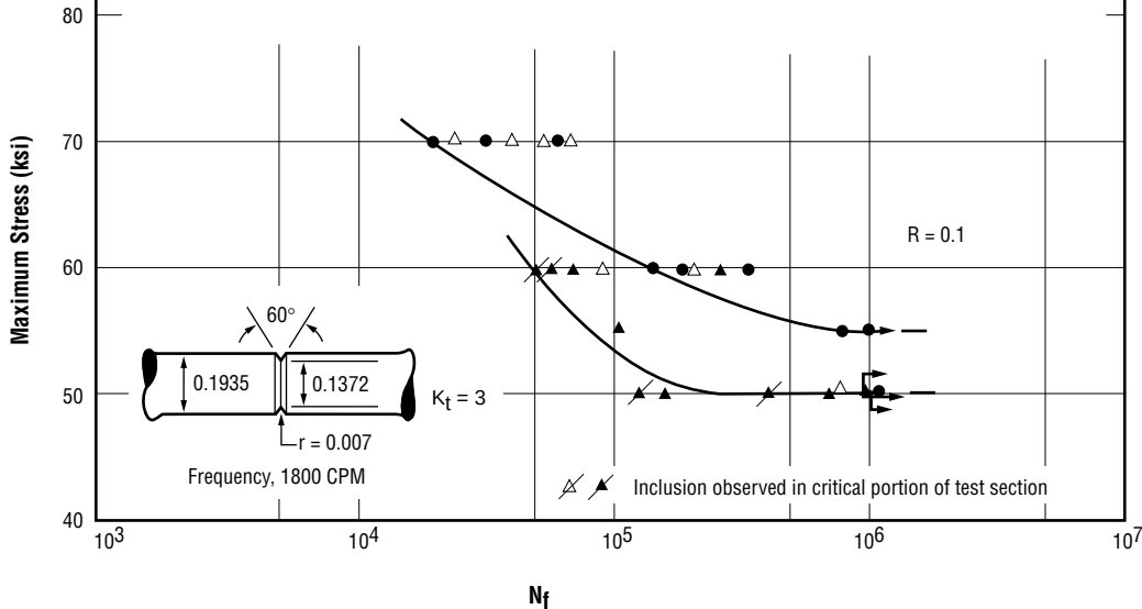
Figure 3.5.1.6 Room temperature mild-notch fatigue properties of annealed and solution treated and aged castings from two casting manufacturers (Ref. 8)
