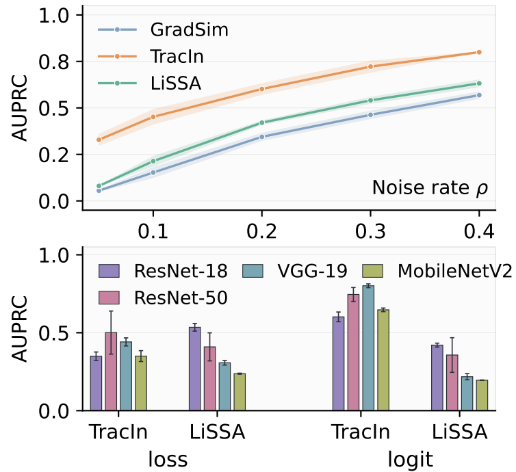
(c) Robustness
