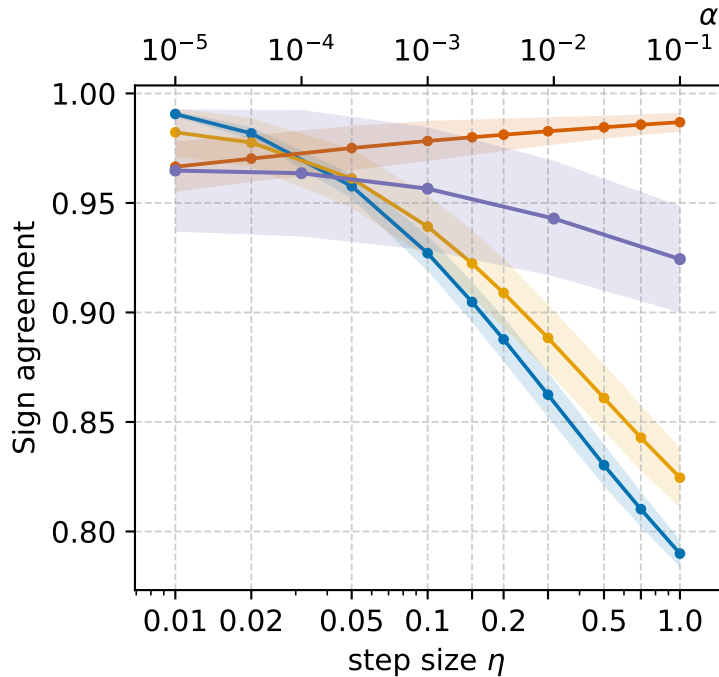
(b) FashionMNIST
