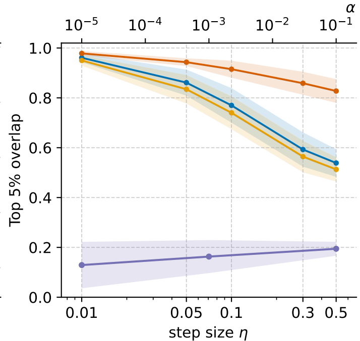
(c) CIFAR-10
