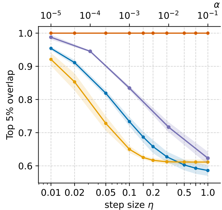
(a) FashionMNIST
