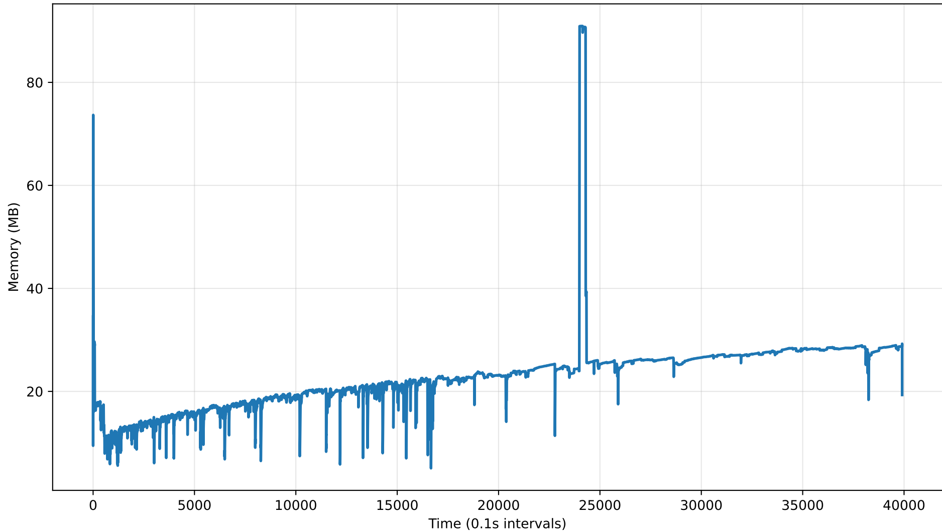
Memory Usage
