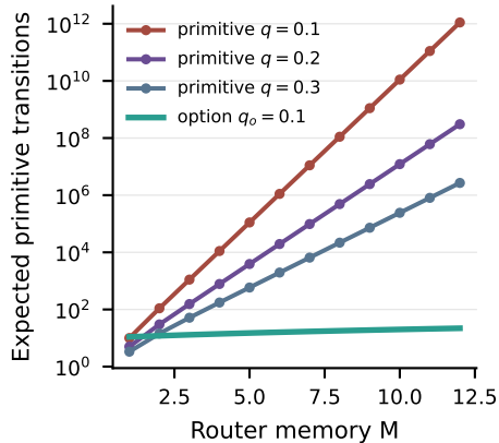
A. Exponential fresh-path gap
