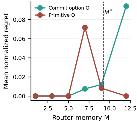
C. Option helps, then overcorrects
