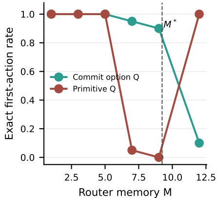
B. Frozen Q-learning sweep
