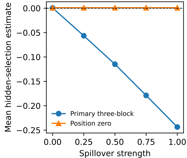
A. Bias under planted carryover
