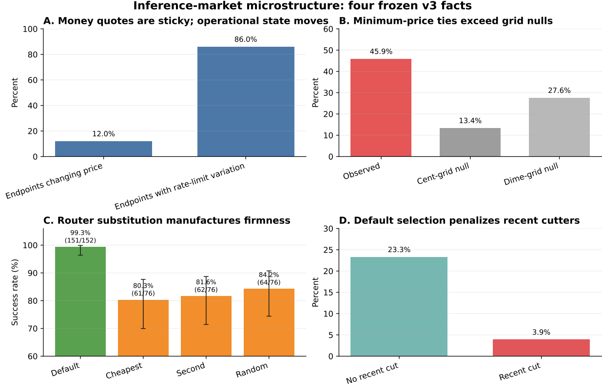
Figure 1: Four frozen v3 facts. Panel C shows marginal Wilson 95% intervals; the registered policy contrasts use block randomization inference at the 500-per-pinned-arm gate. Panels A, B, and D are descriptive panel statistics.
