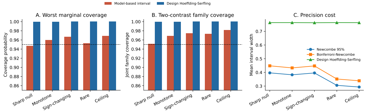
Figure 4: Outcome-blind interval audit over five fixed binary potential-outcome schedules and 3,000 stopped assignments per schedule. Panel A takes the worse coverage of the two primary contrasts; Panel B reports simultaneous family coverage; Panel C shows the precision cost. Bonferroni-Newcombe is descriptive under a binomial model. The wider design-Hoeffding-Serfling interval is valid for the conditional finite population; its observed near-100% coverage is an audit, not the source of its guarantee.
