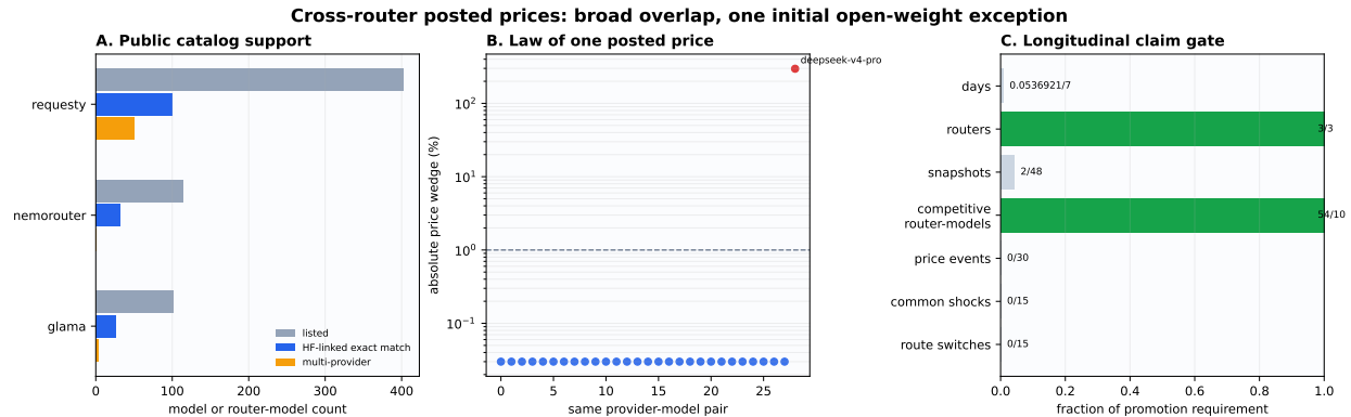
Figure 7: Discovery cross-router posted-price audit. Among 29 Hugging-Face-linked exact provider-model pairs, 28 have identical component prices. The DeepSeek exception is cross-sectional; the right panel records the longitudinal gates. H94 excludes this entire discovery cross-section and uses only snapshots after its 2026-07-17 04:30:20 UTC activation; one eligible snapshot per router is currently present and all event gates remain closed.
